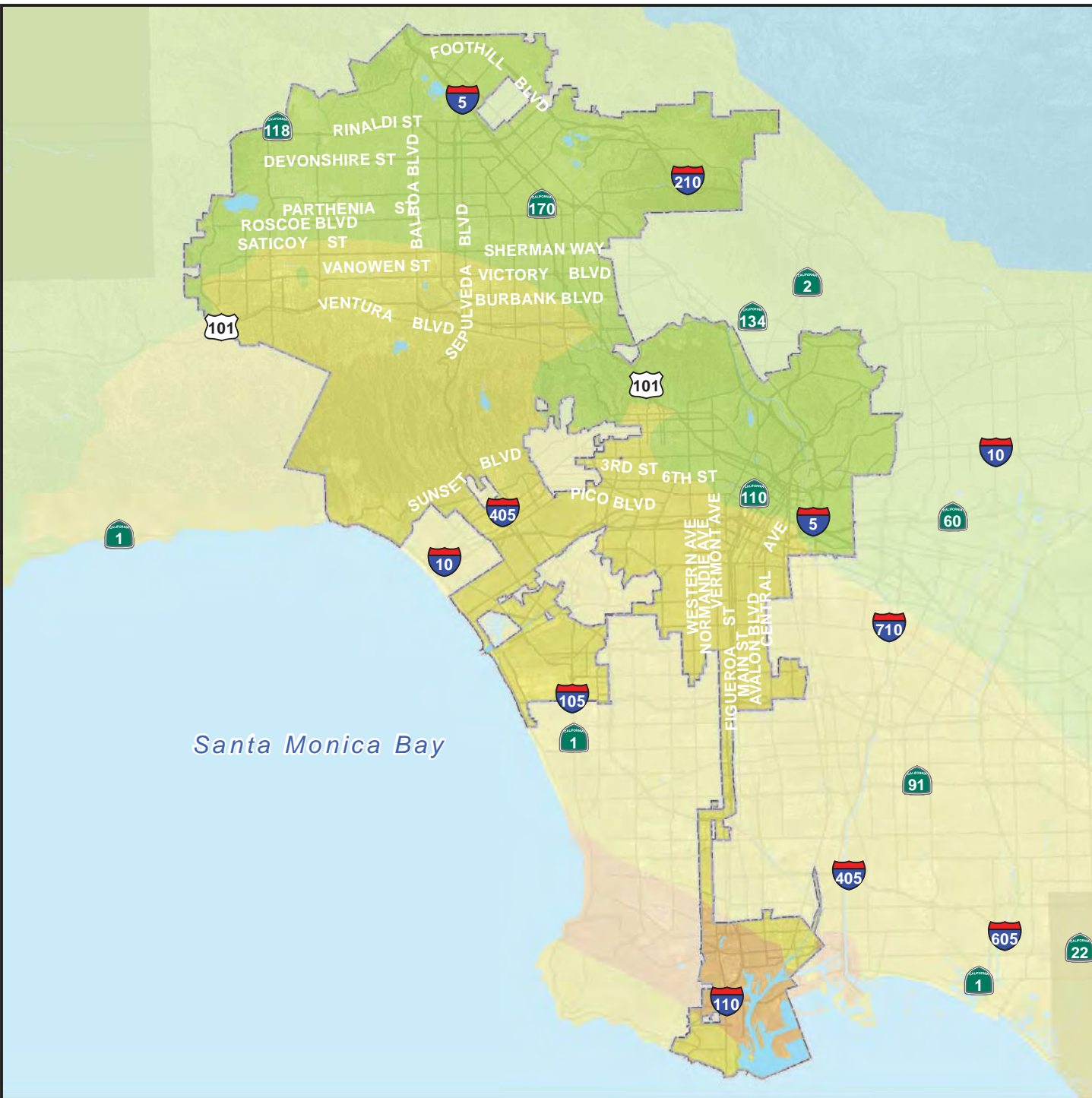
City of Los Angeles Figure 9-4. Palos Verdes M7.3 Earthquake Scenario Peak Ground Acceleration
