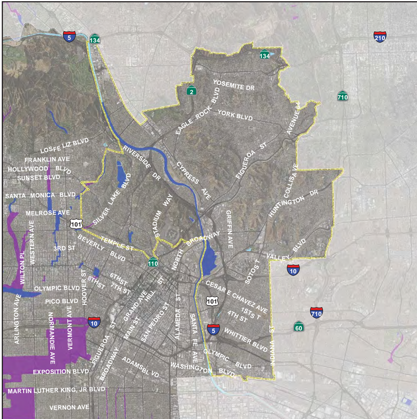
East Los Angeles APC Figure 10-2. FEMA DFIRM Flood Hazard Areas
