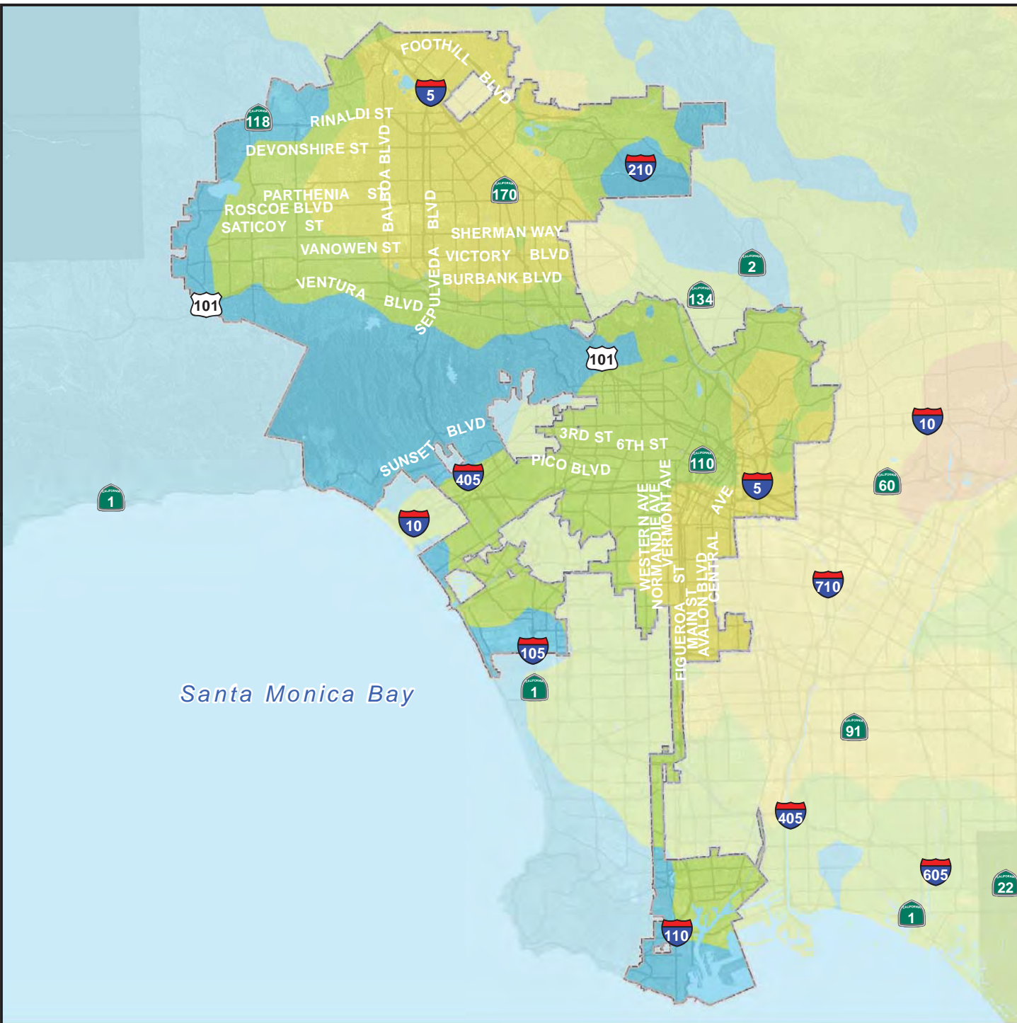
City of Los Angeles Figure 9-6. San Andreas M7.8 Earthquake Scenario Peak Ground Acceleration
