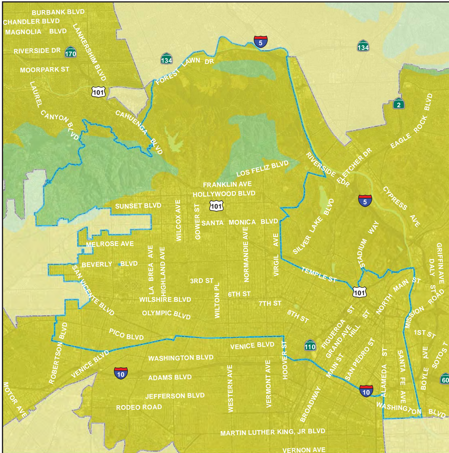
Central APC Figure 9-8. National Earthquake Hazards Reduction Program (NEHRP) Soils
