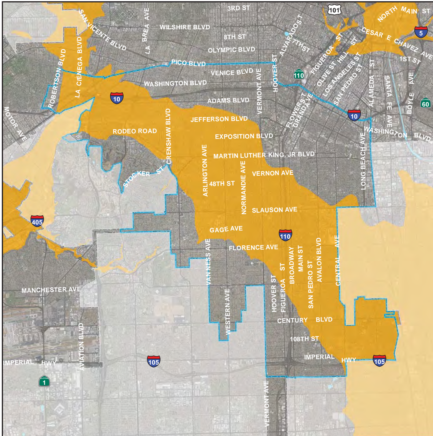
South Los Angeles APC Figure 9-19. Liquefaction Zones
